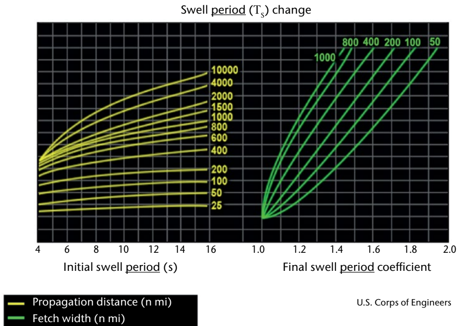
Figure 4.11. Bretschneider swell period decay nomogram. To calculate: choose the initial swell period (in s) on the left horizontal axis, move vertically up to the correct propagation distance line in yellow (in n mi = nautical miles), then horizontally across to the correct fetch width line in green (really defined as fetch length, in n mi), then vertically down to the swell period coefficient. Multiply the initial swell period by this coefficient.
