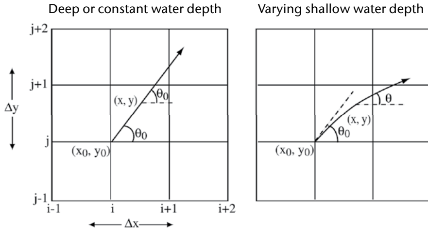
Figure 5.3. Typical grid for numerical wave models ( x stands for x_1 and y for x_2 ). In grid-type models, the energy in (f, \theta) bins is propagated between points according to an equation like Equation 5.4. In ray models, the energy is followed along characteristic lines.
