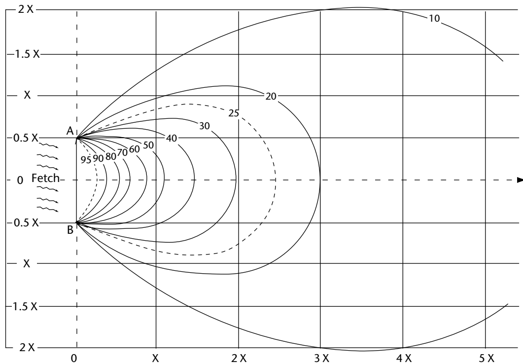
Figure 3.3. Possible directions for swell originating at a storm front AB and incident on a point P
