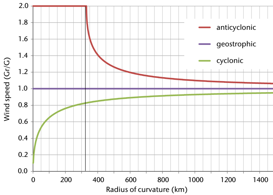
Figure 2.15. Ratio of gradient wind speed to geostrophic wind for anticyclonic and cyclonic flows at latitude 40°N. Geostrophic wind speed is 15 knots in this example. The black solid line marks the area of no winds around a pressure high. For numeric values of gradient wind, see Tables 2.4 and 2.5.
