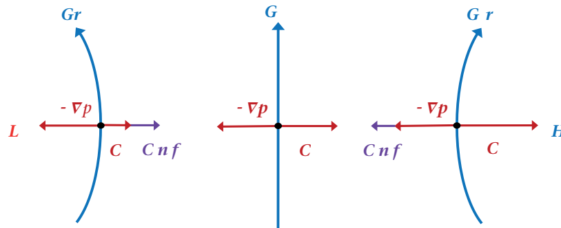
Figure 2.16. Balance of forces for basic types of frictionless flow (northern hemisphere) (C = Coriolis force, Cnf = centrifugal force, G = geostrophic wind, Gr = gradient wind, H = high-pressure centre, L = low-pressure centre and -\nabla p = pressure gradient force)
