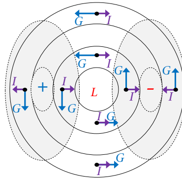
Figure 2.19. Example of the isallobaric wind field of a moving low-pressure system. Solid line = isobar, dashed line = isallobar, G = (u_g, v_g) = geostrophic wind, L = low-pressure centre and I = (u_i, v_i) = isallobaric wind, which is always directed towards areas of pressure decrease. This results in a wind decrease/increase north/south of the depression. Wind direction is affected in the front and rear of the system.
