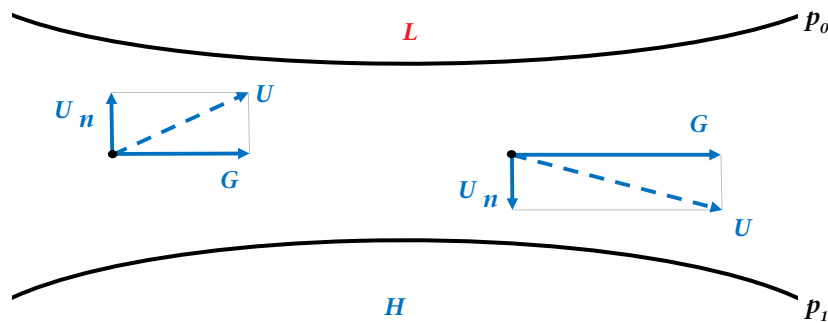
Figure 2.20. Examples of confluent/diffluent wind fields ( p_0 and p_1 are isobars, U_n is the non-geostrophic wind component, G and U are the geostrophic and surface winds, H = high-pressure centre and L = low-pressure centre)
