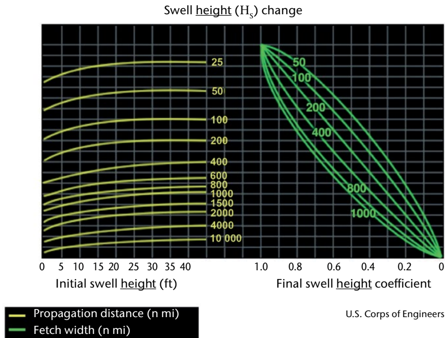
Figure 7. Bretschneider swell height decay nomogram. To calculate: choose the initial swell height (in feet) on the left horizontal axis, move vertically up to the propagation distance line in yellow (in nautical miles (n mi)), then horizontally across to the correct fetch width line in green (really defined as fetch length, in n mi), then vertically down to the swell height coefficient. Multiply the initial swell height by this coefficient.
