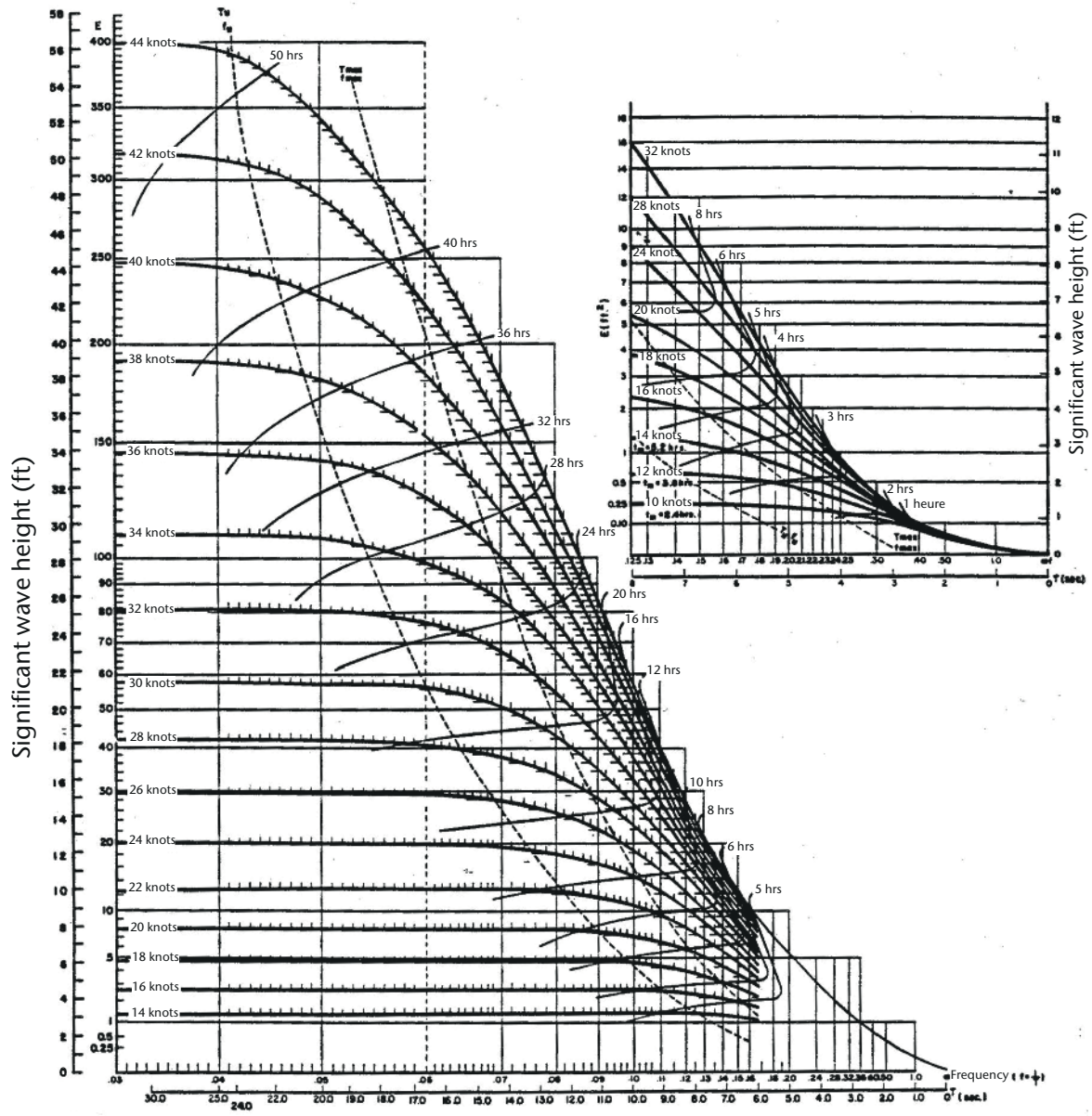
Figure 3. Duration graph: distorted co-cumulative spectra for wind speeds from 10 to 44 knots versus duration
