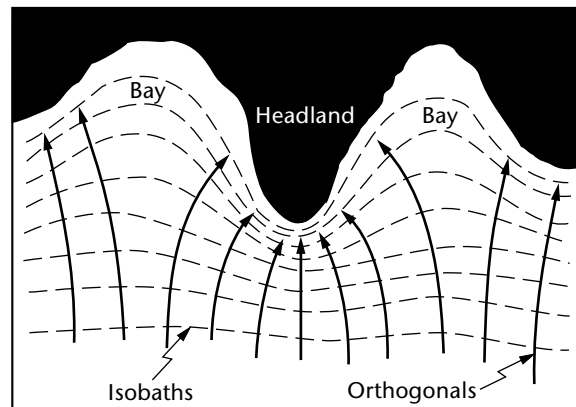
Figure 1.8. Refraction along an irregular shoreline
