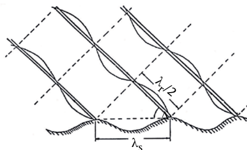
Figure 7.3. Bragg diffraction of radio waves from a sinusoidal sea wave. Conditions for constructively interfering backscatter from successive crests.
