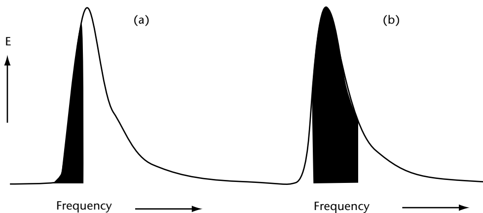
Figure 3.5. Effect of dispersion on waves leaving a fetch, showing the spectrum at the fetch front. The first components to arrive at a point far downstream constitute the shaded part of the spectrum in (a). Higher frequencies arrive later, by which time some of the fastest waves (lowest frequencies) have passed by as illustrated in (b).
