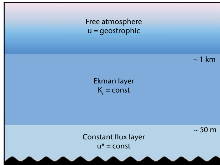
Figure 2.6. Schematic of the two-regime boundary layer; u is the horizontal wind speed and u_* is the friction velocity representing the turbulent vertical momentum flux
