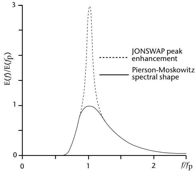
Figure 1.17. General form of a JONSWAP spectrum as a function of f/f_p
