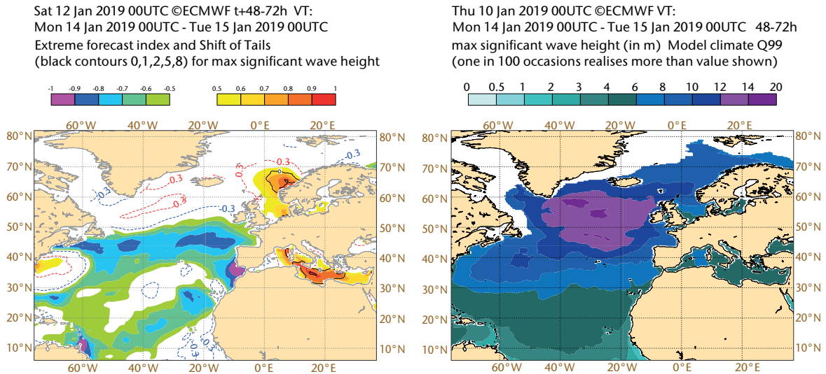
Figure 6.13. EFI (left panel) and associated ninety-ninth percentile of significant wave height derived from the model's long-term climate simulation (right panel)
