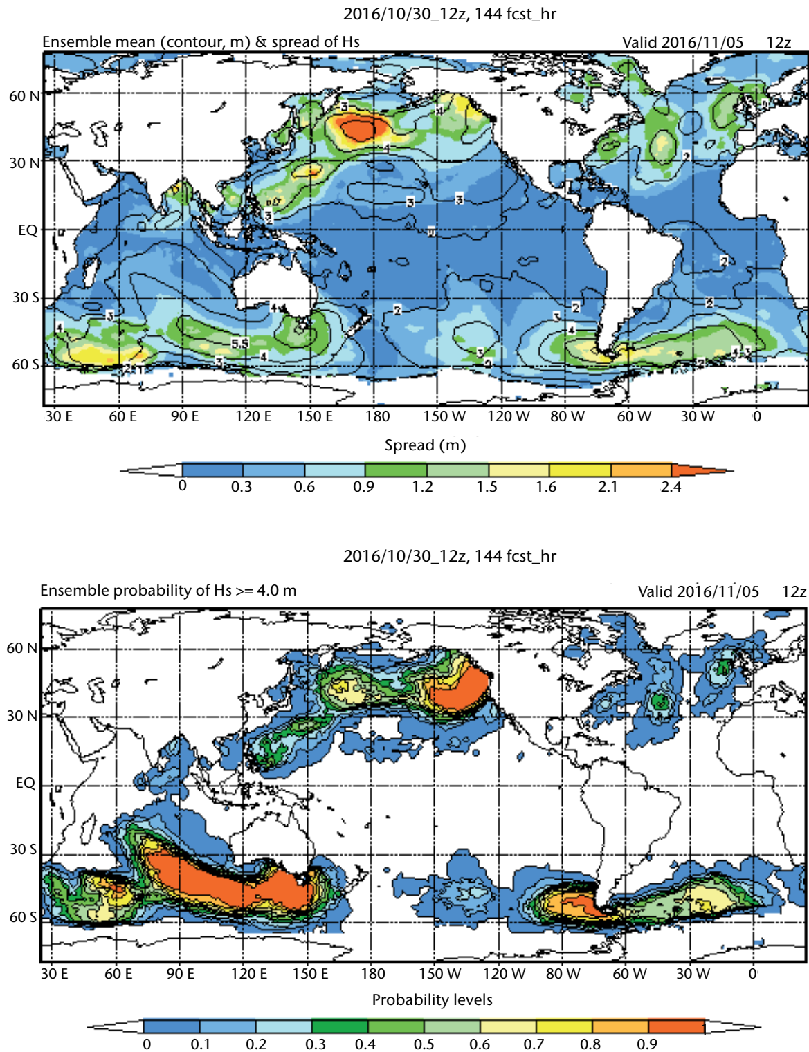
Figure 6.11. Ensemble forecast charts showing (top) ensemble mean significant wave height (contours) and spread (shading), and (bottom) probability of significant wave height exceeding 4 m
