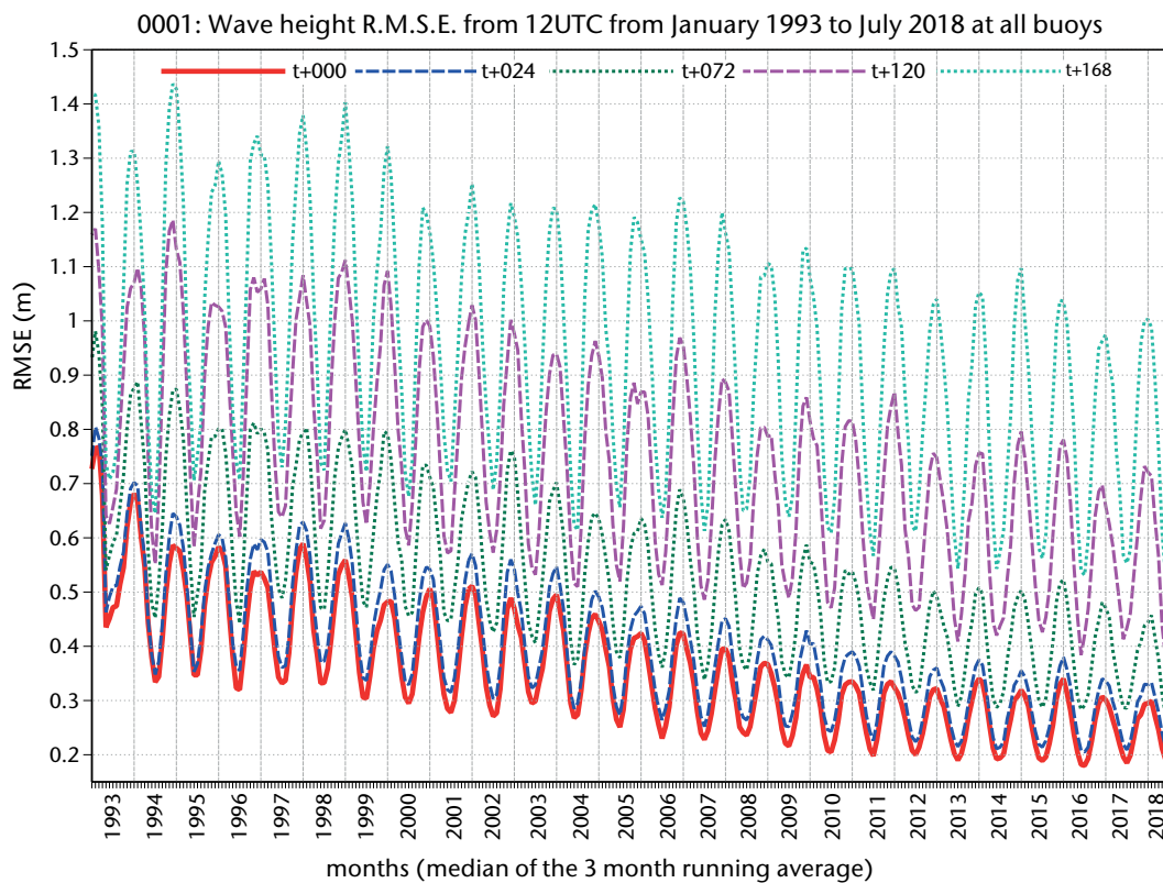
Figure 6.8. Year by year change in RMSE scores for ECMWF global wave-model forecasts of significant wave height referenced against a global network of in situ wave-measurements platforms
