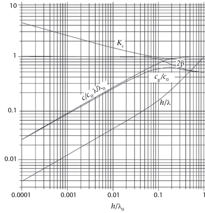
Figure 4.12. Illustration of various functions of h/\lambda_0
