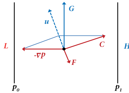
Figure 2.17. Balances of friction, pressure gradient and Coriolis forces (northern hemisphere) ( C = Coriolis force, F = friction, G = geostrophic wind, H = high-pressure centre, L = low-pressure centre, -\nabla p = pressure gradient force and u = surface wind; p_0 and p_1 represent isobars)
