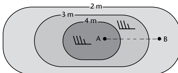
Figure 4.5. Wave field at time t_0 indicated by lines of equal wave height
