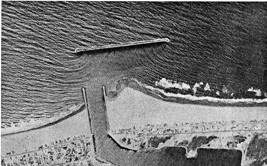
Figure 1.9. Wave diffraction at Channel Islands harbour breakwater (California)
