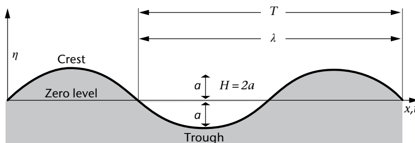
Figure 1.2. A simple sinusoidal wave
