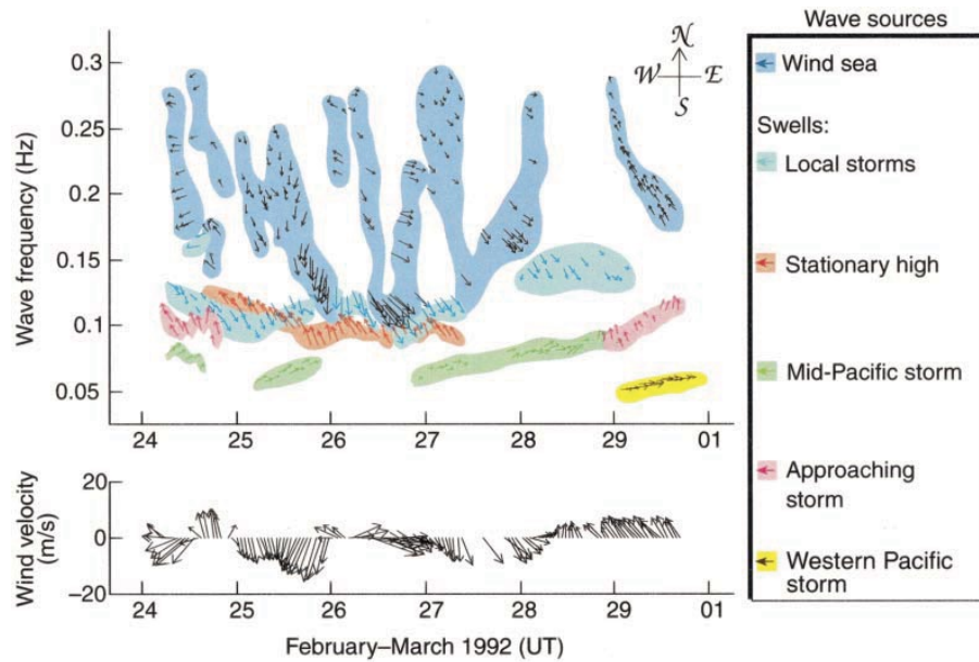
Figure 6.2. Clustering of partitioned wave data in time series. The diagram shows evolution of data from a complex sea comprising short-period (high-frequency) wind seas superimposed on moderate- to long-period swells generated in other parts of the ocean basin.
