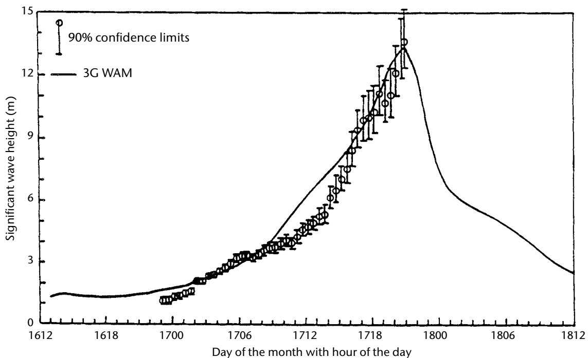
Figure 5.5. Comparison of calculated and observed wave heights during Hurricane Camille (1969). The wave sensor failed at the height of the storm.
