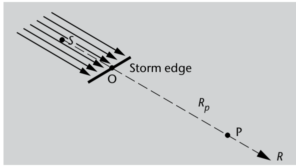
Figure 4.8. Swell from a quasi-stationary, distant storm, in which the waves travel over a distance R , and the generation area has a long fetch
