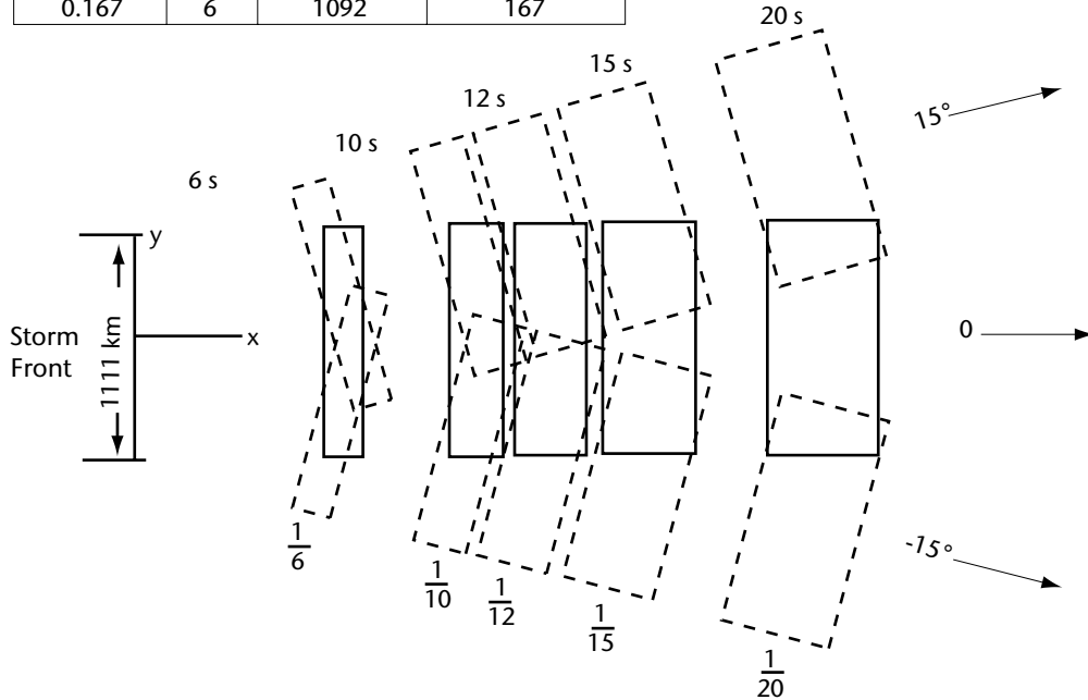
Figure 5.4. Propagation of discrete spectral components from a storm front. This illustrates the effects of angular spreading and dispersion on the wave energy. The garden sprinkler effect resulting from the discretization of the spectrum can be seen.
