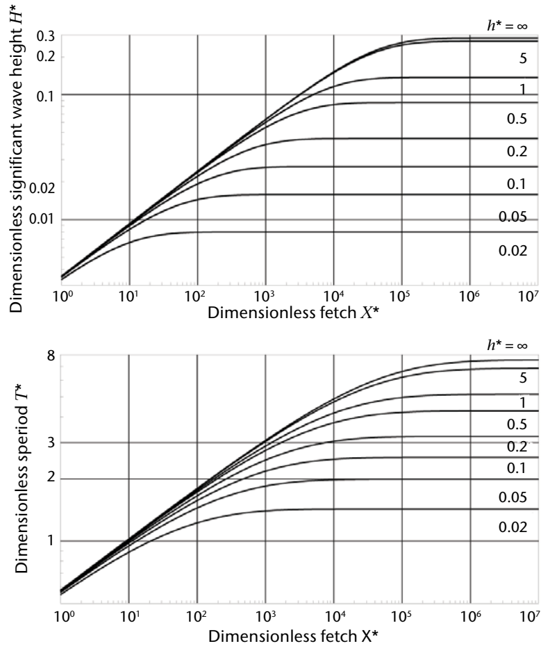
Figure 3.2. Shallow-water growth curves for dimensionless significant wave height (upper) and period (lower) as functions of fetch, plotted for a range of depths
