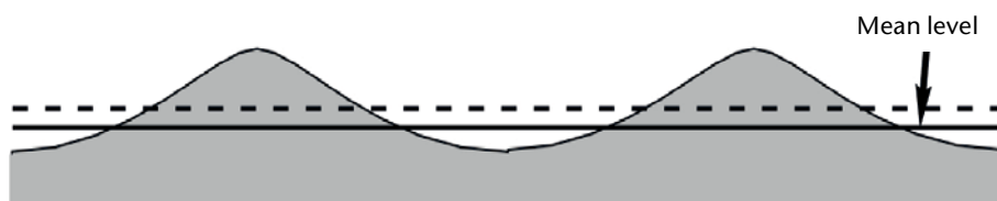
Figure 1.10. Trochoidal wave profile; the crests project farther above the mean level than the troughs sink under it
