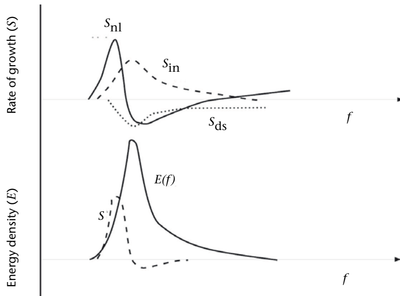
Figure 3.6. Growth from non-linear interactions ( S_{nl} ) as a function of frequency for the mean JONSWAP spectrum ( E )
