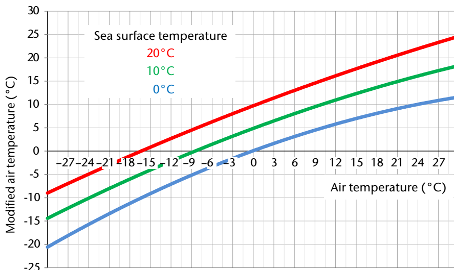
Figure 2.10. Modification of air temperature in 2 m over water after 120 min of advection.
