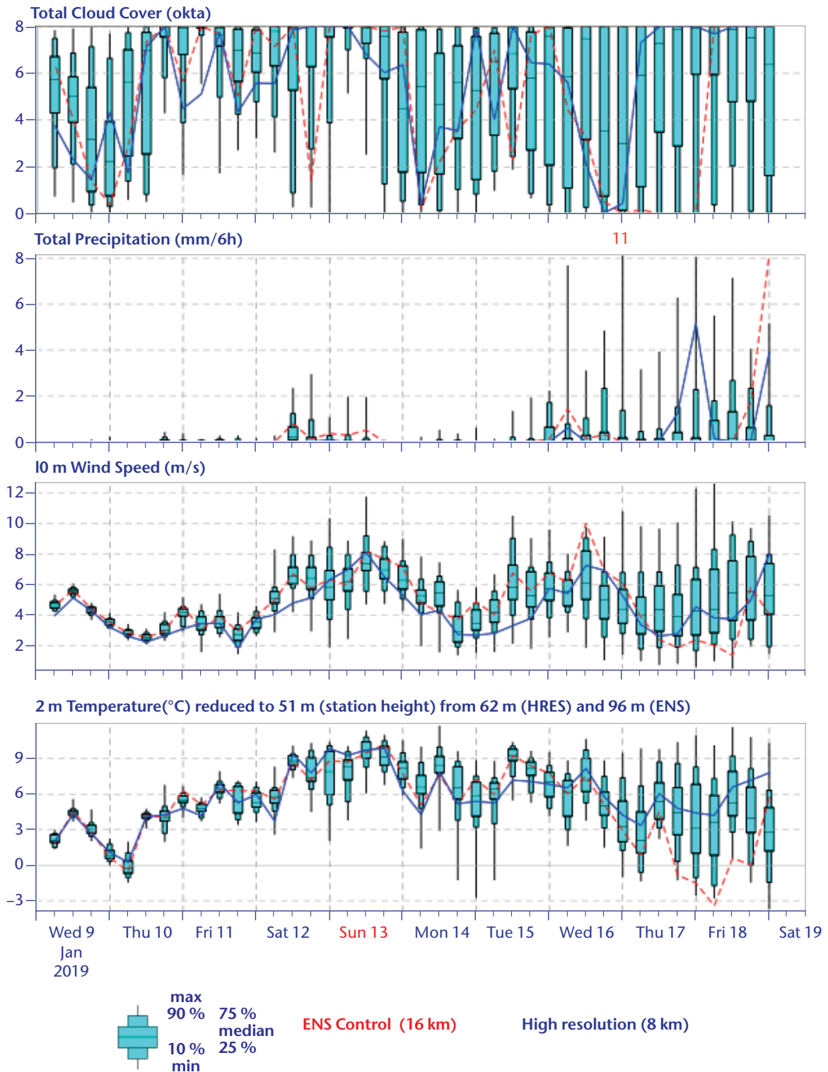
Figure 2.24. Example of an ENS meteogram comparing the high-resolution model run (blue curves) with the frequency distribution of 50 ensemble runs and the undisturbed control run (red curves)
