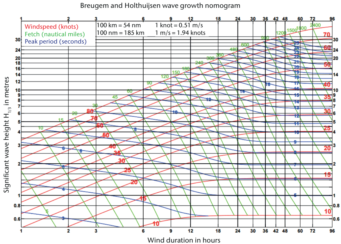
Figure 4.1. Manual wave-growth nomogram
