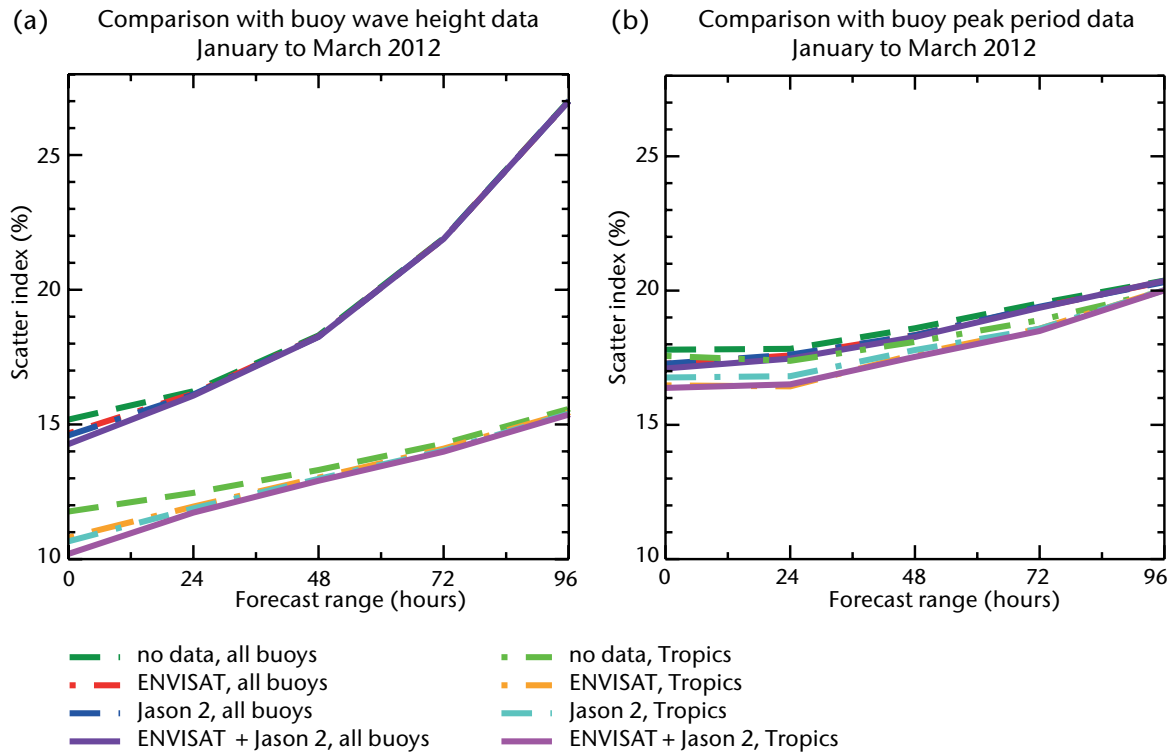
Figure 5.2. Impact of using altimeter wave-height data in a global model analysis. Verification is made against all available buoy data and buoy data from the tropics for wave height (a) and peak period (b). A set of 3 months stand-alone runs at 28 km resolution, forced by operational analysis winds were performed: a reference run with no data, one with Envisat data, another one with Jason-2 data and a final run with Envisat and Jason-2 data. Scatter index is the standard deviation of the difference normalized by the mean of the observations
