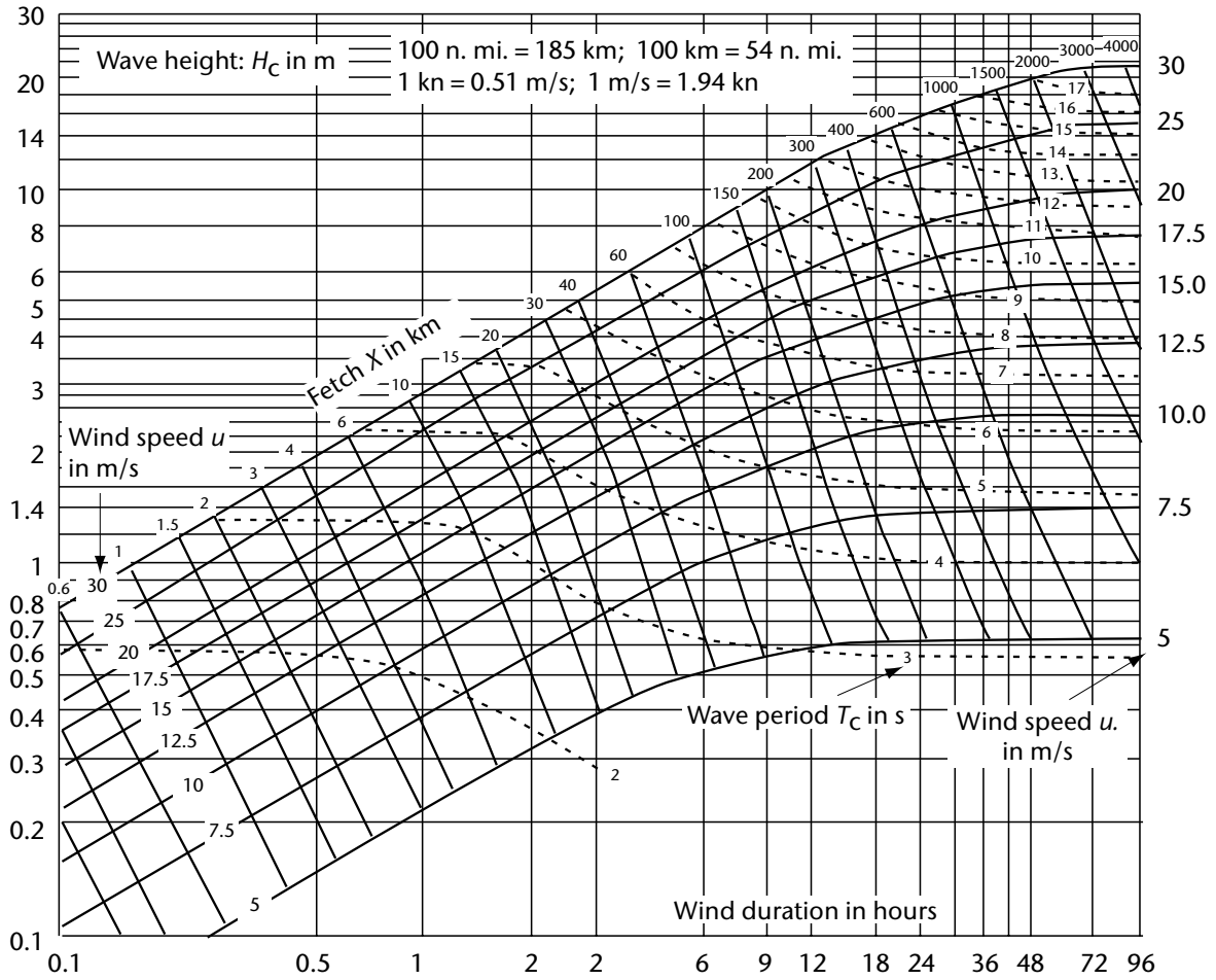
Figure 2. Manual wave forecasting diagram (kn = knots; n. mi. = nautical miles)
