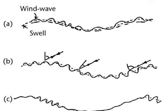
Figure 7.4. Mechanisms of spatial modulation by long gravity waves of radar scattering from capillary waves: (a) straining and velocity modulation of short wind waves by longer wind waves and swell, (b) tilt modulation and (c) roughness modulation
