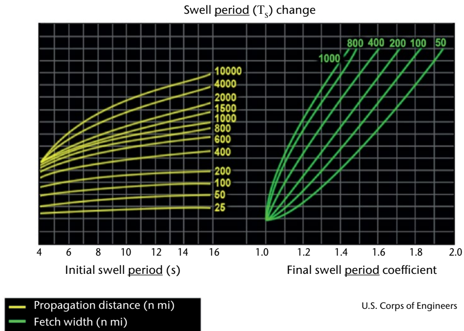
Figure 8. Bretschneider swell period decay nomogram. To calculate: choose the initial swell period (in s) on the left horizontal axis, move vertically up to the correct propagation distance line in yellow (in n mi), then horizontally across to the correct fetch width line in green (really defined as fetch length, in n mi), then vertically down to the swell period coefficient. Multiply the initial swell period by this coefficient.
