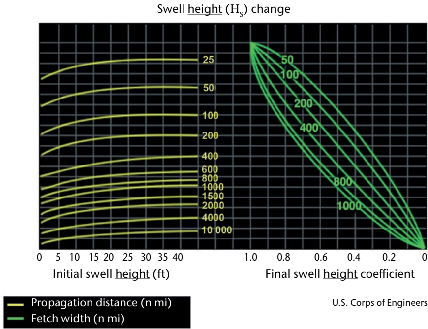
Figure 4.10. Bretschneider swell height decay nomogram. To calculate: choose the initial swell height(in feet) on the left horizontal axis, move vertically up to the propagation distance line in yellow (in n mi = nautical miles), then horizontally across to the correct fetch width line in green (really defined as fetch length, in n mi), then vertically down to the swell height coefficient. Multiply the initial swell height by this coefficient.
