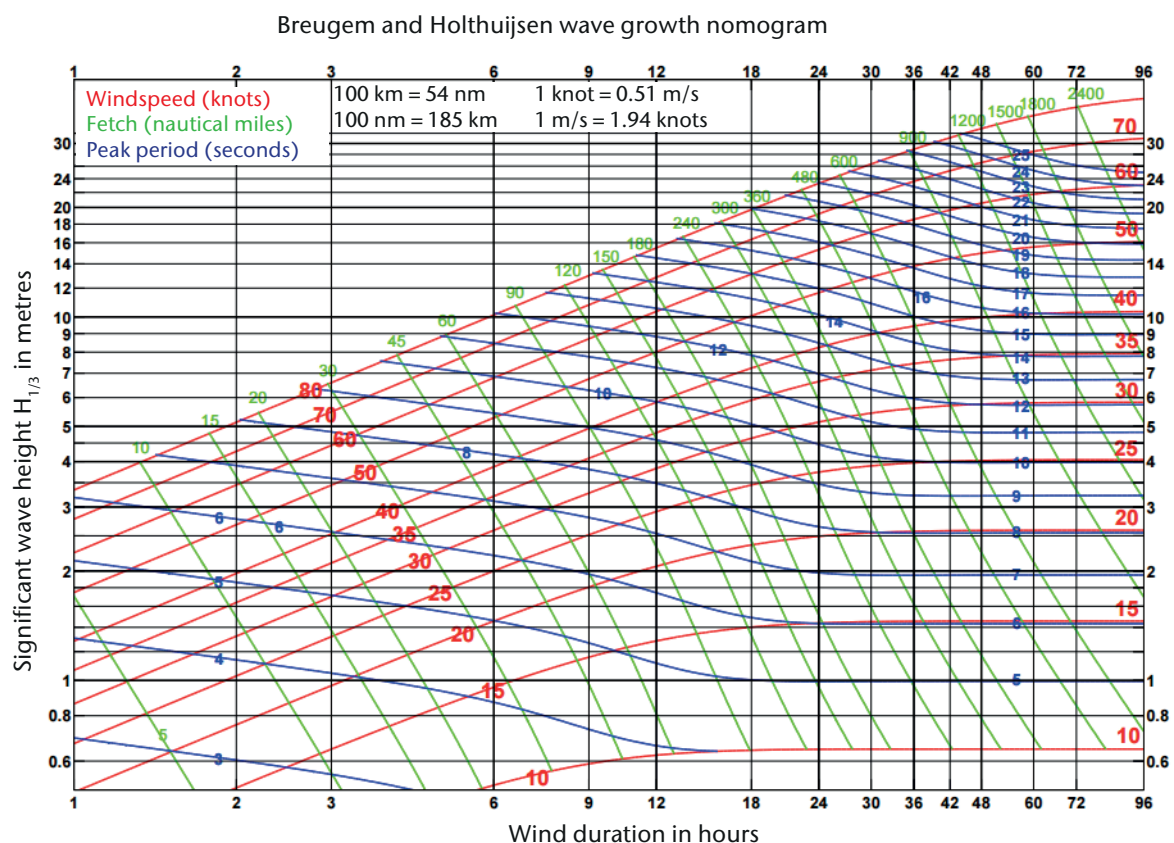
Figure 1. Manual wave growth nomogram
